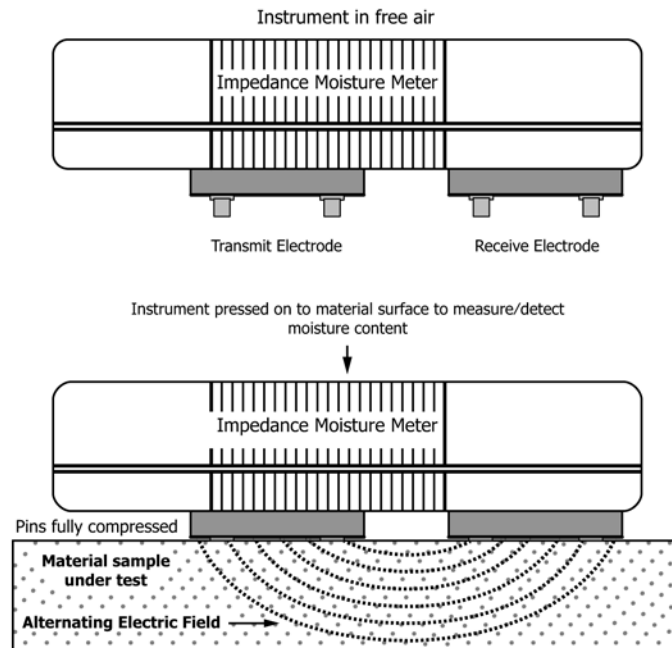
FIG. X2.1 Typical Moisture Meters for Concrete and Other Floor Slabs Showing: Electrodes and Positioning on Surface of the Floor Slab
